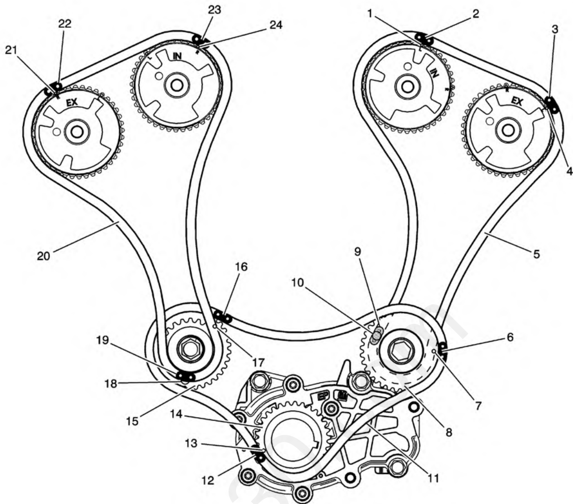
Fig. 4: Locating Stage Two Timing Marks Courtesy of GENERAL MOTORS COMPANY
